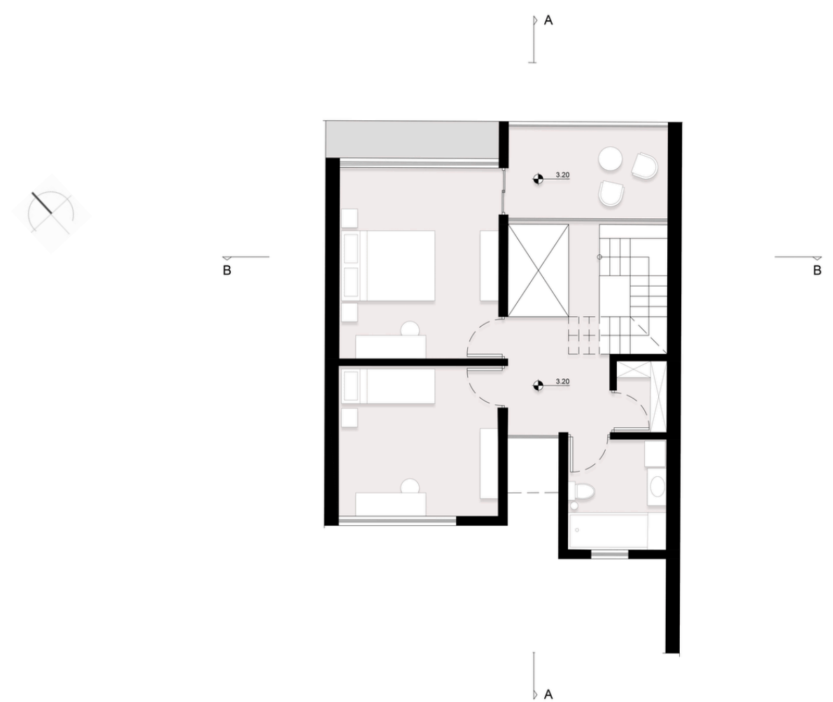
ΚΑΤΟΨΗ Α' ΟΡΟΦΟΥ
